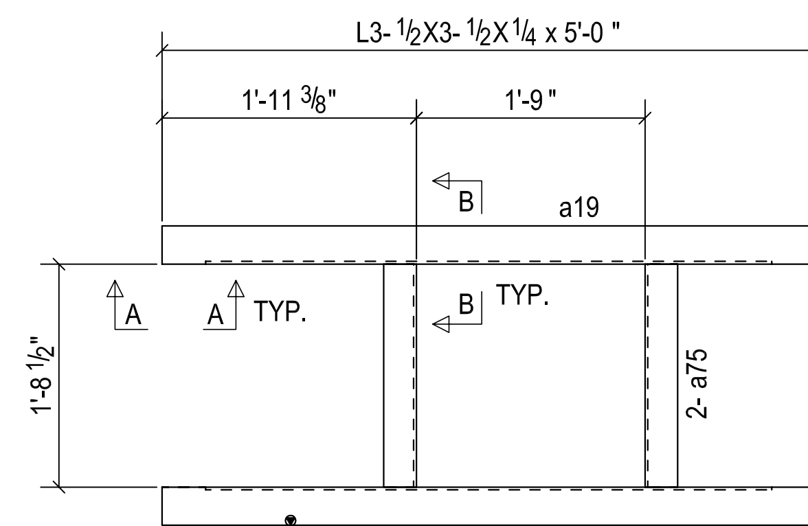
ONE - ROOF FRAMING - 116FR2
