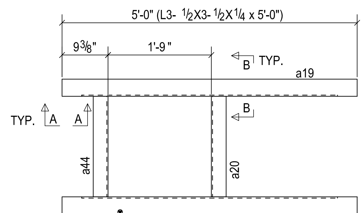
2 - ROOF FRAMINGS - 116FR1
